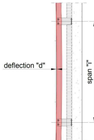
Image 7 – The maximum deflection of the battens/profiles between two brackets d_{max} must be \leq 1/200 for the span between the brackets "l"
