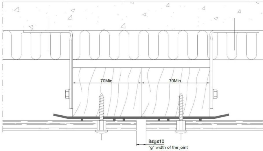
Image 25 - Example of a horizontal section of the ventilated facade package along a vertical joint between panels. Note the protective gasket and the minimum width of the wooden battens.
