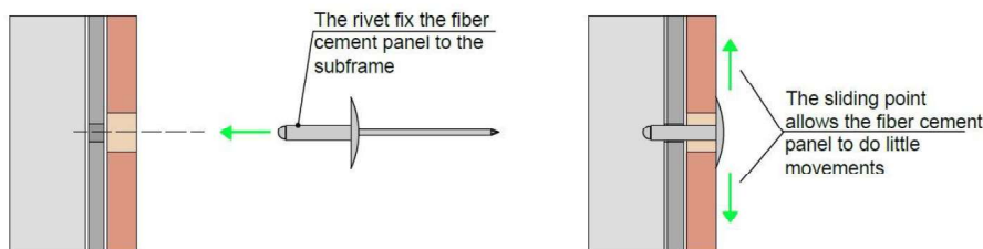
Image 21 - Example of steps to fix Opus Profiber-cement panels. The panels are pre-drilled with holes that all have the same diameter of 9.5 mm. The example shows how the diameters of the holes for the fixed points are reduced using suitable metal bushings.
