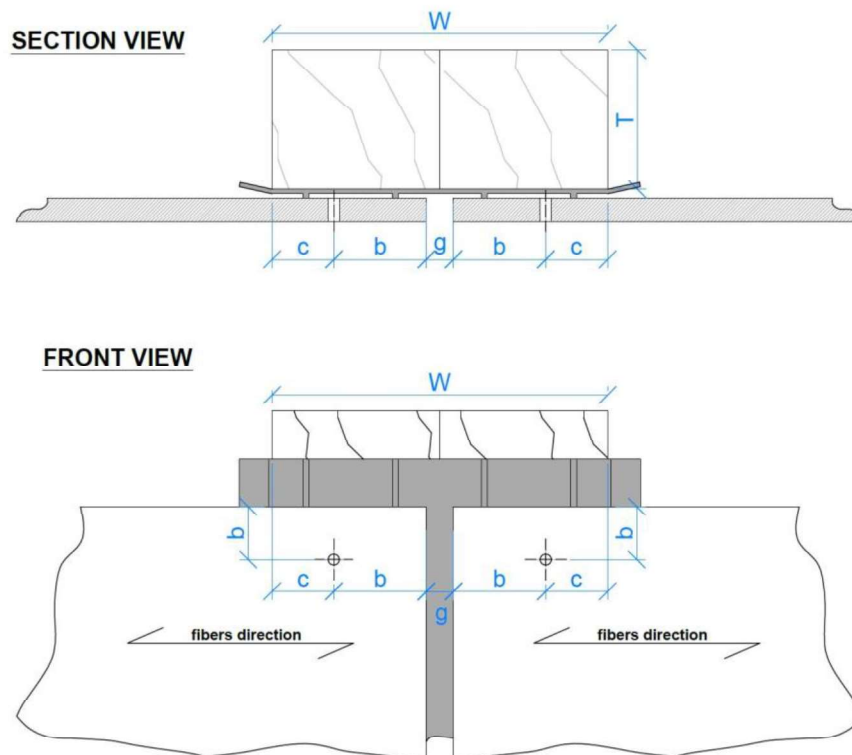
Image 11 – Geometrical specifications of the cladding required to determine the width of the wooden beams of the subframe
