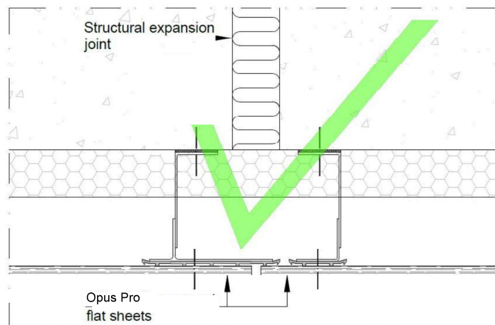
Image 10– Horizontal sections – Examples of incorrect and correct arrangement of profiles and cladding panels along an expansion joint of the supporting structure
