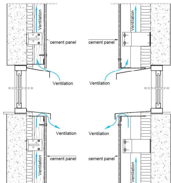
Image 24 - Example of a section of a ventilated facade package along a window. Wooden subframe on the left and aluminum subframe on the right, both cladded with Opus Pro fiber-cement flat panels
