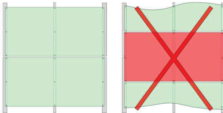
Image 23 - Left: example of a correct way to secure Opus panels, with the horizontal joint of the cladding aligning with the expansion joint of the subframe profiles. Right: example of an incorrect way to secure the Silbonit panels, with a cladding sheet secured to two profiles.
