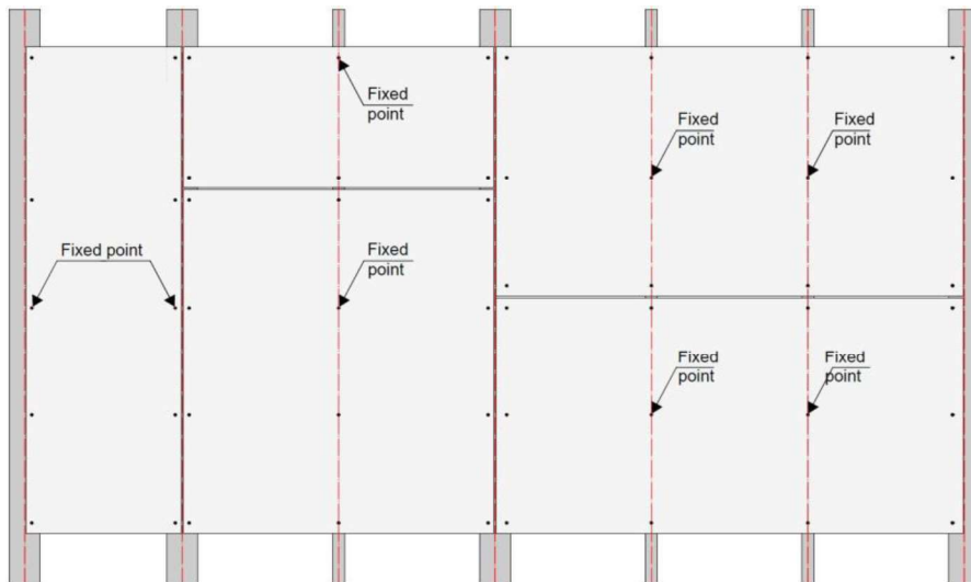
Image 19- Example of cladding with Opus Pro fiber-cement panels. In some cases, the geometry of the panel and the facade layout may require two fixed points.
