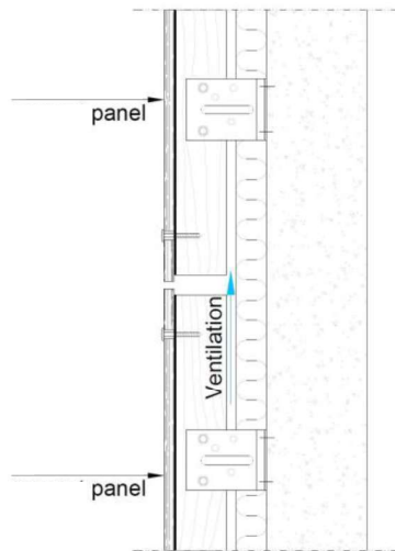
Image 26 - Example of a vertical section of the ventilated facade package along a horizontal joint between panels. Wooden subframe and Opus Pro fiber-cement flat-panel cladding.
